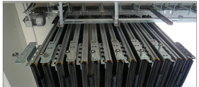
Door leave stacked at 90° to the opening and held in position by the slim-line top track
